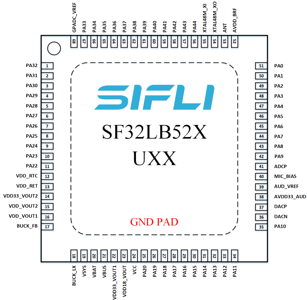
Figure 5-2: SF32LB52x Pin Layout
